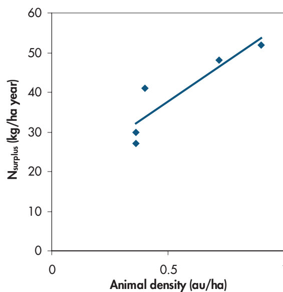
Figure 2-15. Average animal density and surplus of nitrogen per ha and year for the three years period for all the Finnish F-BERAS-farms.
