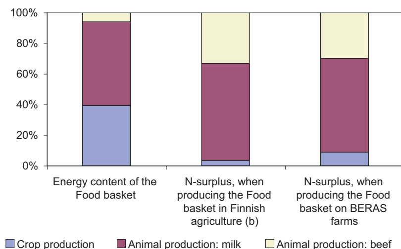
Figure 9-6. Energy content (J) of the Food basket (50 % of the Finnish food energy consumption) and nitrogen (N) surplus (kg) of the Food basket production by two production lines: average Finnish agriculture (b= surplus based on the production lines: crop and animal production) and BERAS-farms, relative scale %.
